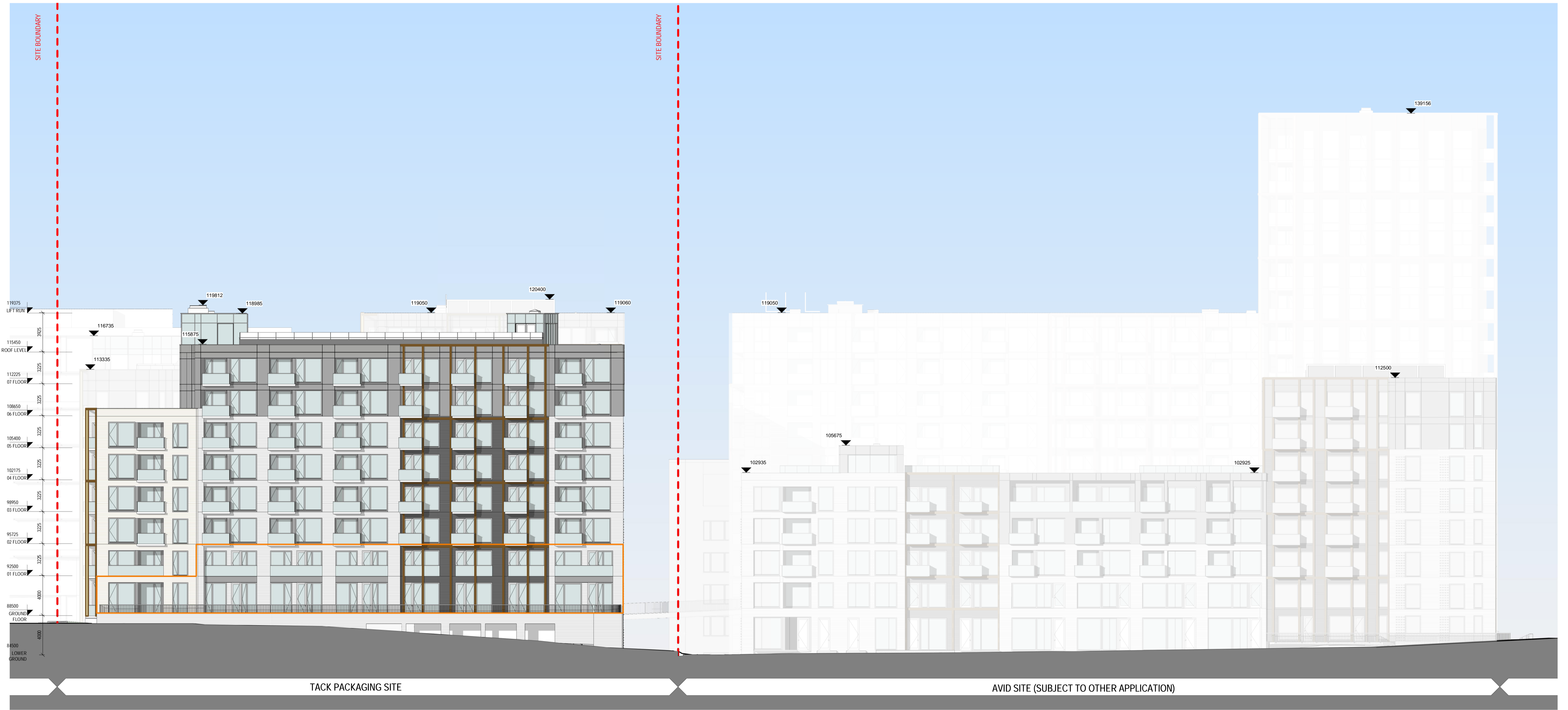
1 PROPOSED SOUTH WEST ELEVATION - TACK SITE 1:200
